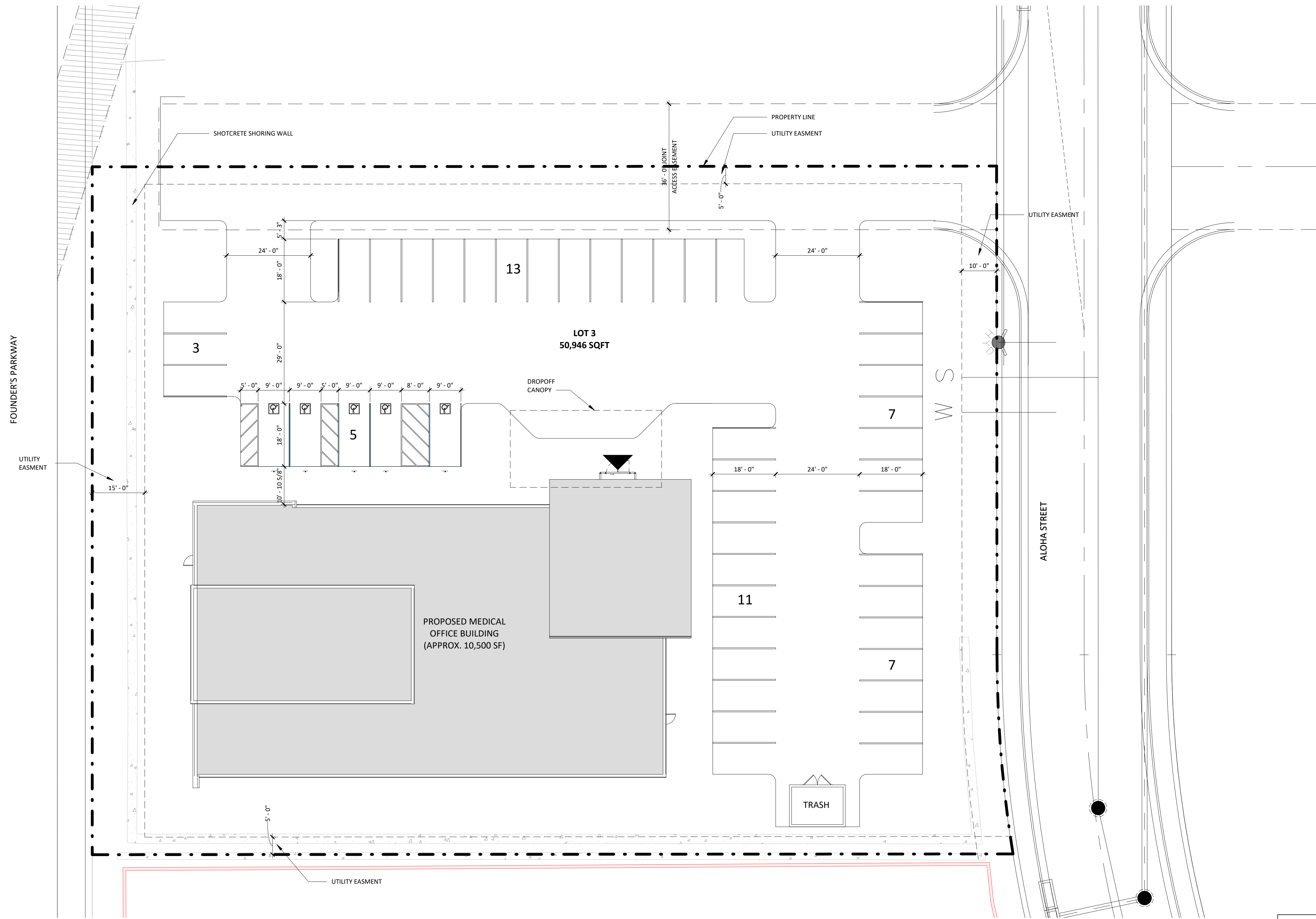
1 SITE PLAN A3.1 | A1.10 | 1/16" = 1'-0"
