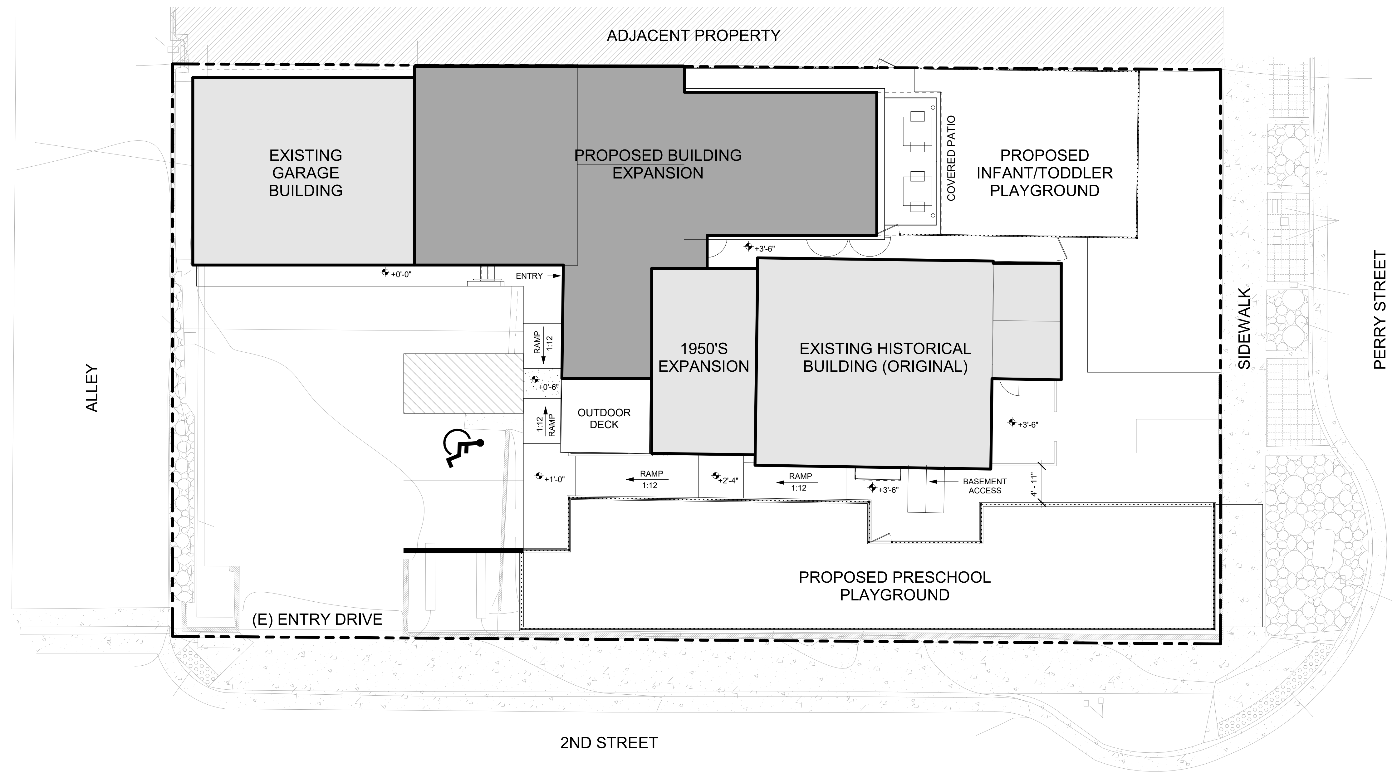
1 CONCEPTUAL SITE PLAN SK1.0 SCALE: 1/8" = 1'-0"
